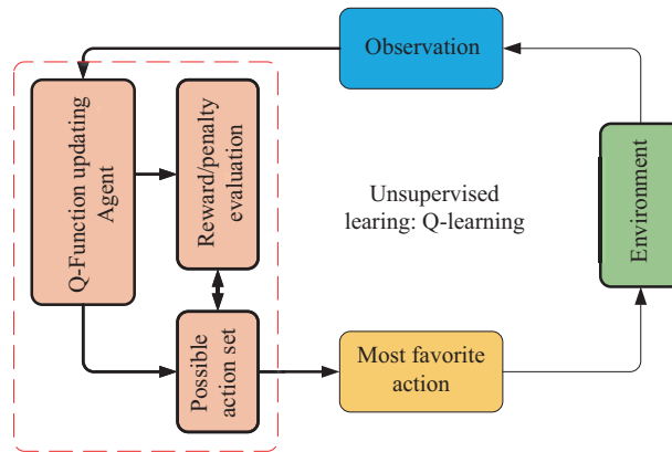
图 3 (网络版彩图) 增强学习示例: Q 学习算法 Figure 3 (Color online) Example of reinforcement learning: Q-learning
